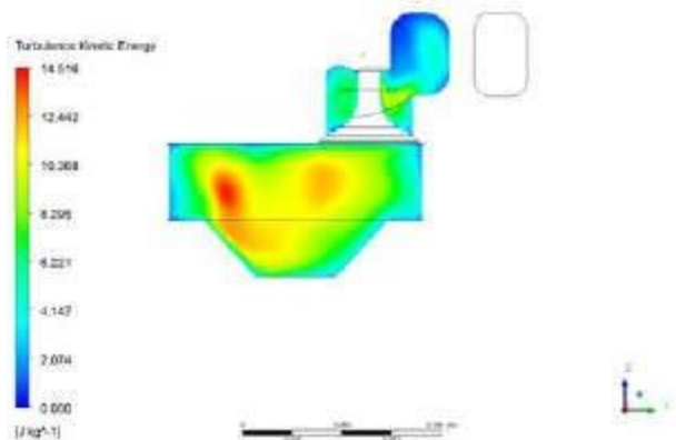
Turbulent kinetic energy at 240 0 crank angle
